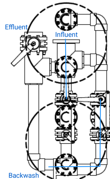
Backwash Mode
