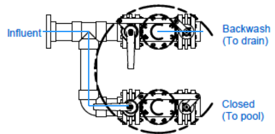
Backwash Mode
