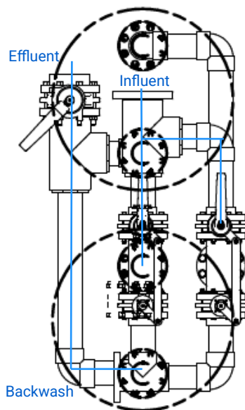
Filter Mode
